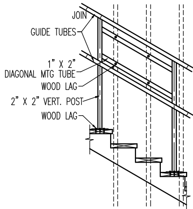
MOUNTING TO STUDS USING DIAGONAL MOUNTING TUBES
