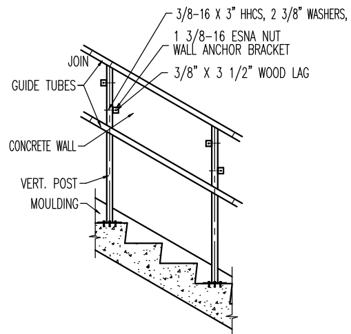
MOUNTING TO CONCRETE WALL WITH MOULDING OR STRINGER PROTRUSION
