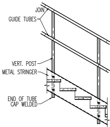
MOUNTING TO SIDE OF STEEL STRINGER
