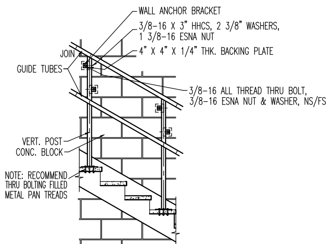
MOUNTING TO CONCRETE BLOCK WALL USING WALL ANCHOR BRACKETS
