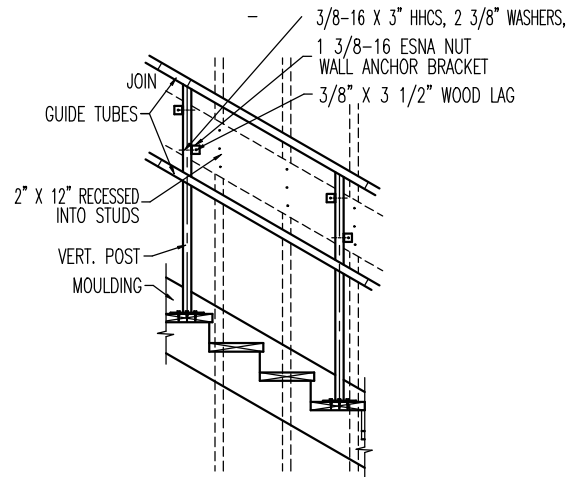
MOUNTING TO RECESSED 2\"/>
