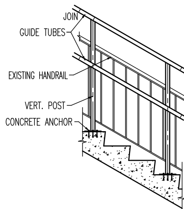
FREE STANDING TRACK MOUNTED DIRECTLY TO TREADS
