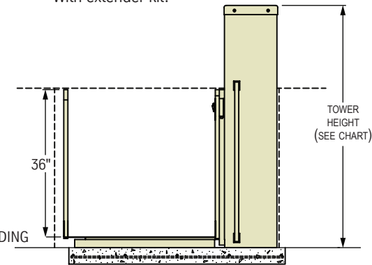
LOWER LANDING SIDE ELEVATION
