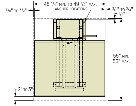
FLOOR & SHAFTWAY LAYOUT
